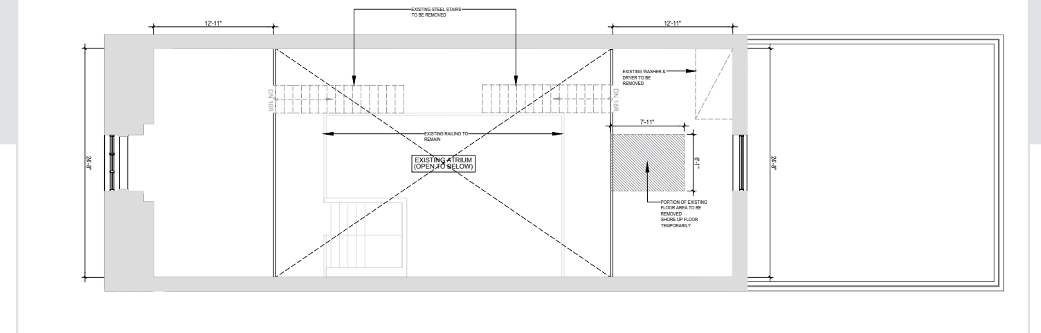
UPPER MEZZANINE DEMOLITION PLAN
