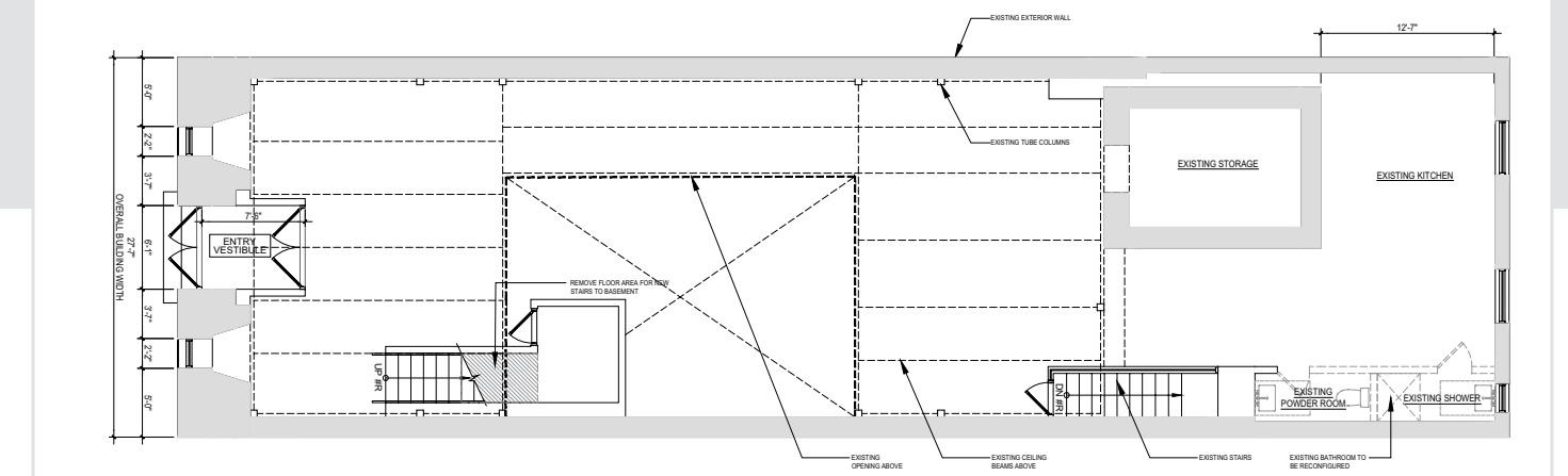
FIRST FLOOR DEMOLITION PLAN
